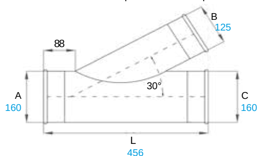
Quick-Fit Standard Branch, 30°
