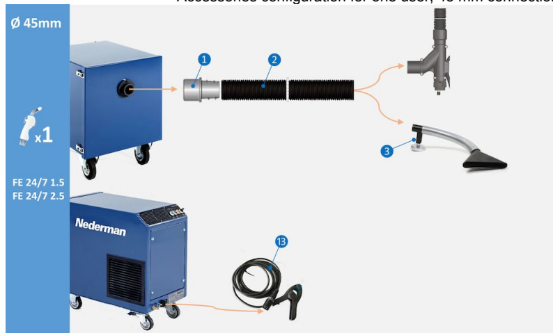
Accessories configuration for one user, 45mm welding machine connection.
